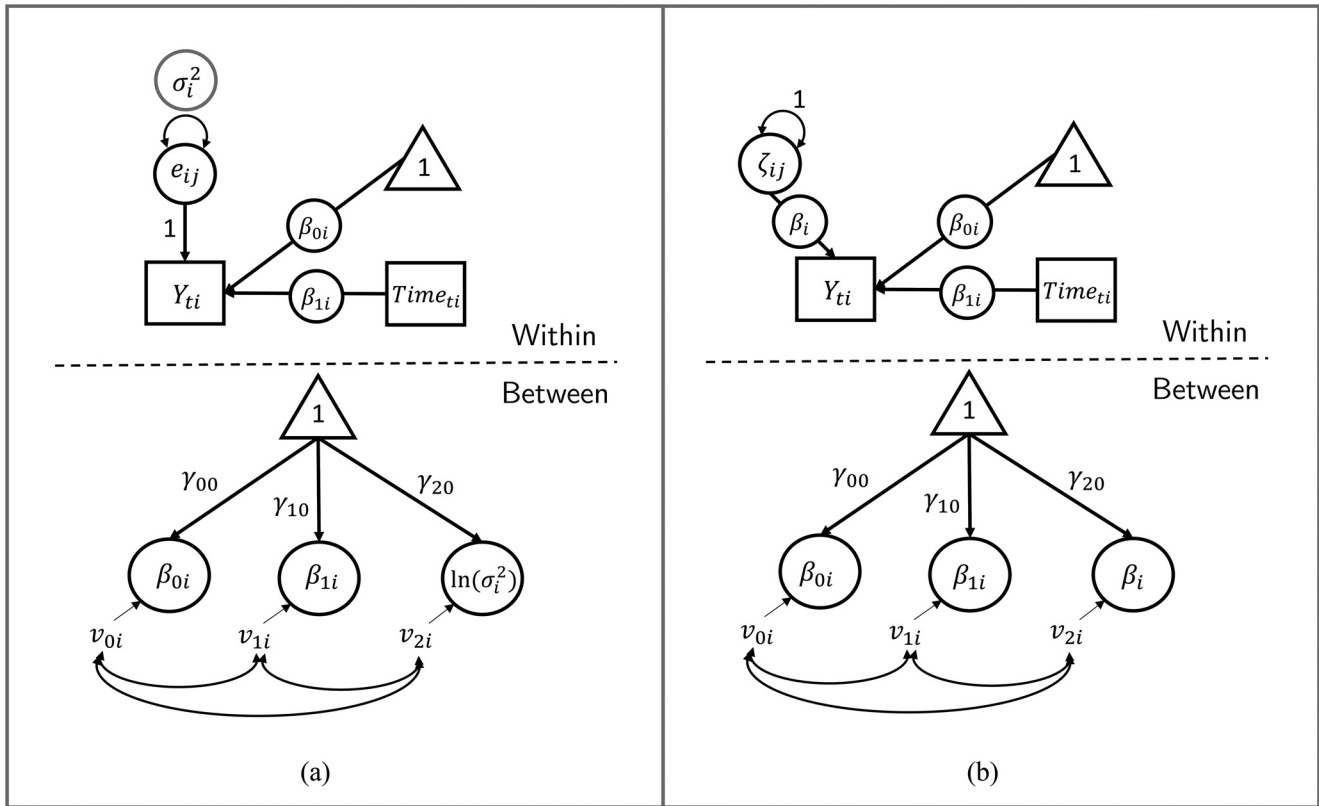
Figure 3 Random Variability Structural Model With One Continuous Observed Outcome Variable Y, Controlling for the Linear Trend Over Time
