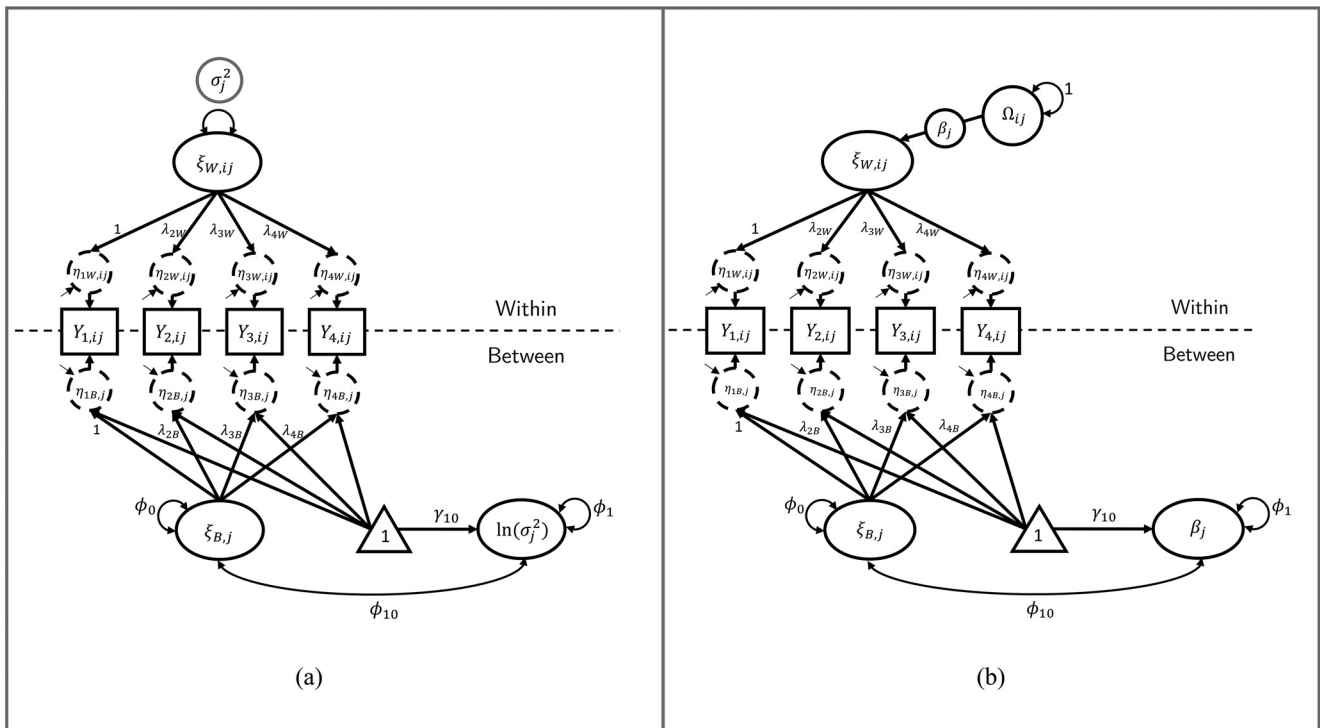
Figure 2 Random Variability SEM With One Within-Level Latent Outcome Variable \xi_W and One Between-Level Latent Outcome Variable \xi_B
