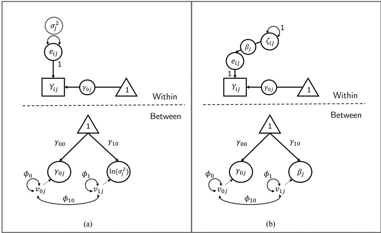
Figure 1 Random Variability Structural Model With One Continuous Observed Outcome Variable Y
