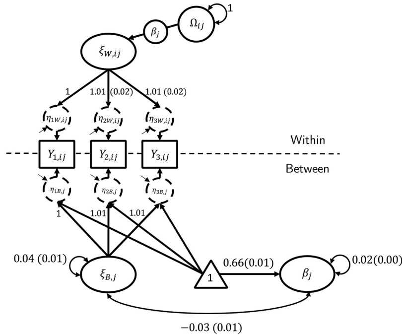
Figure 10 Multilevel Structural Equation Model With Random Scaling Factor Fitted to the PISA 2012 Data, Assessing the Variation Between Schools Regarding Within-School Heterogeneity in Student Perceived Support From Math Teachers
