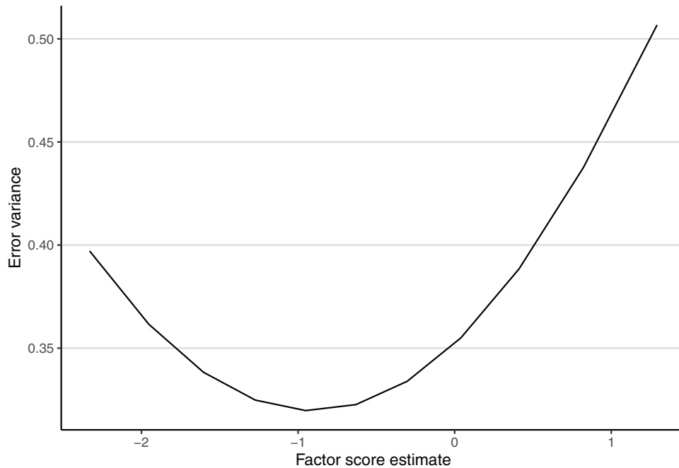
Figure A1 Error Variance of Factor Score Is Not Constant With Categorical Data
