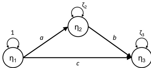
Figure 6 Mediation Model for Study 3
