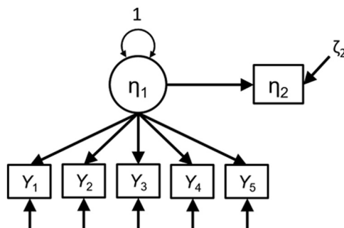
Figure 1 Full SEM Specification of Linear Regression With a Latent Predictor and an Observed Outcome
