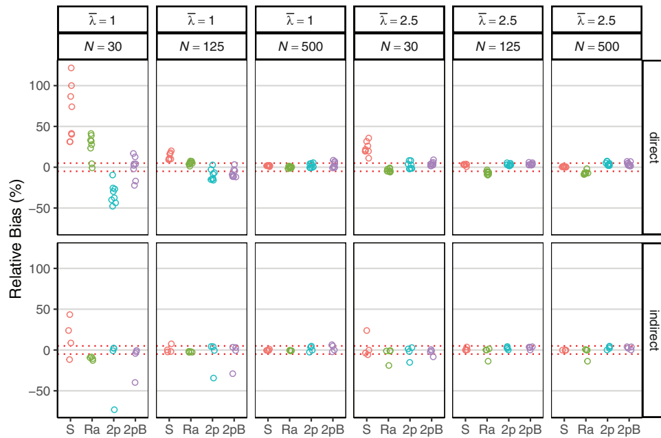
Figure 7 Percentage Relative Bias of Nonzero Direct ( a = .39 , b = .39 , and c = .15 ) and Indirect Effects ( ab = .39^2 ) in Study 3
