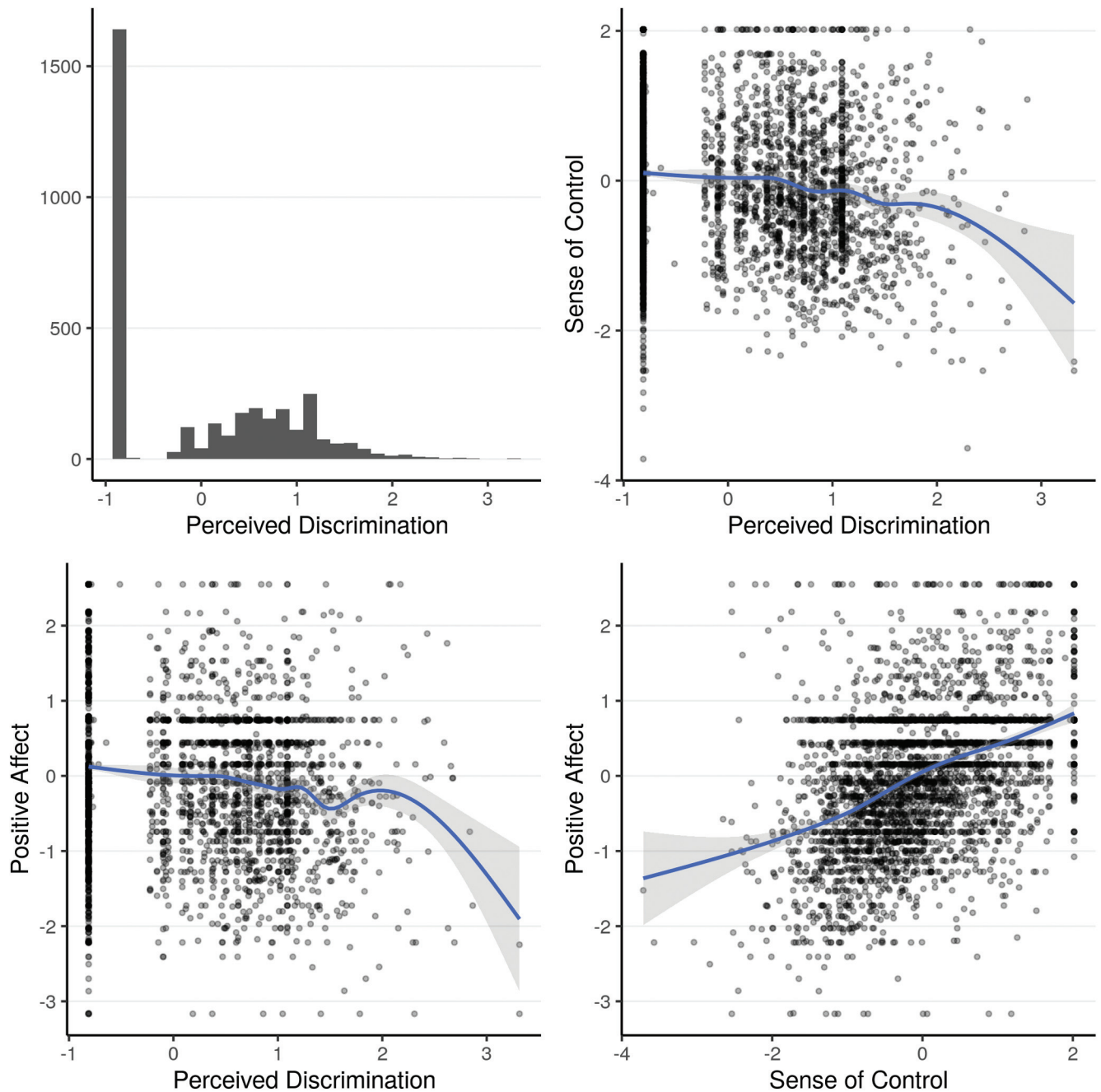
Figure 3 Relations Among Estimated Factor Scores for the Empirical Demonstration
