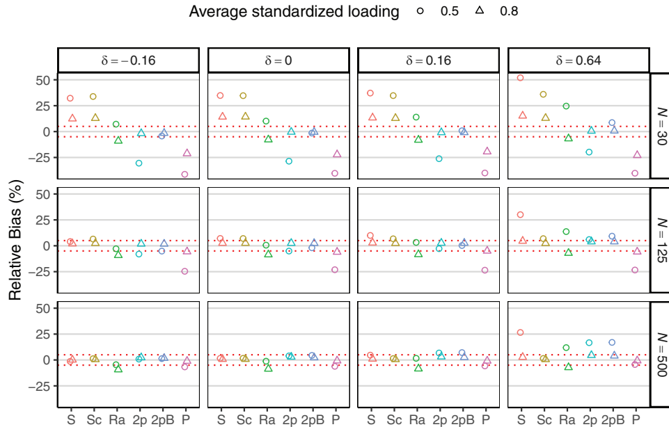
Figure 4 Relative Bias of a Nonzero Path Coefficient in Study 2
