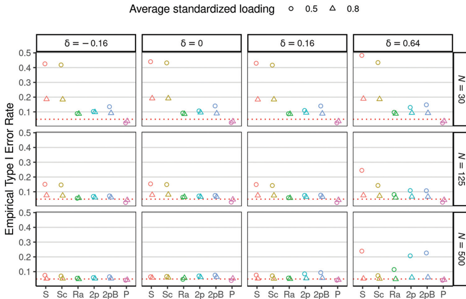
Figure 5 Empirical Type I Error Rates in Study 2
